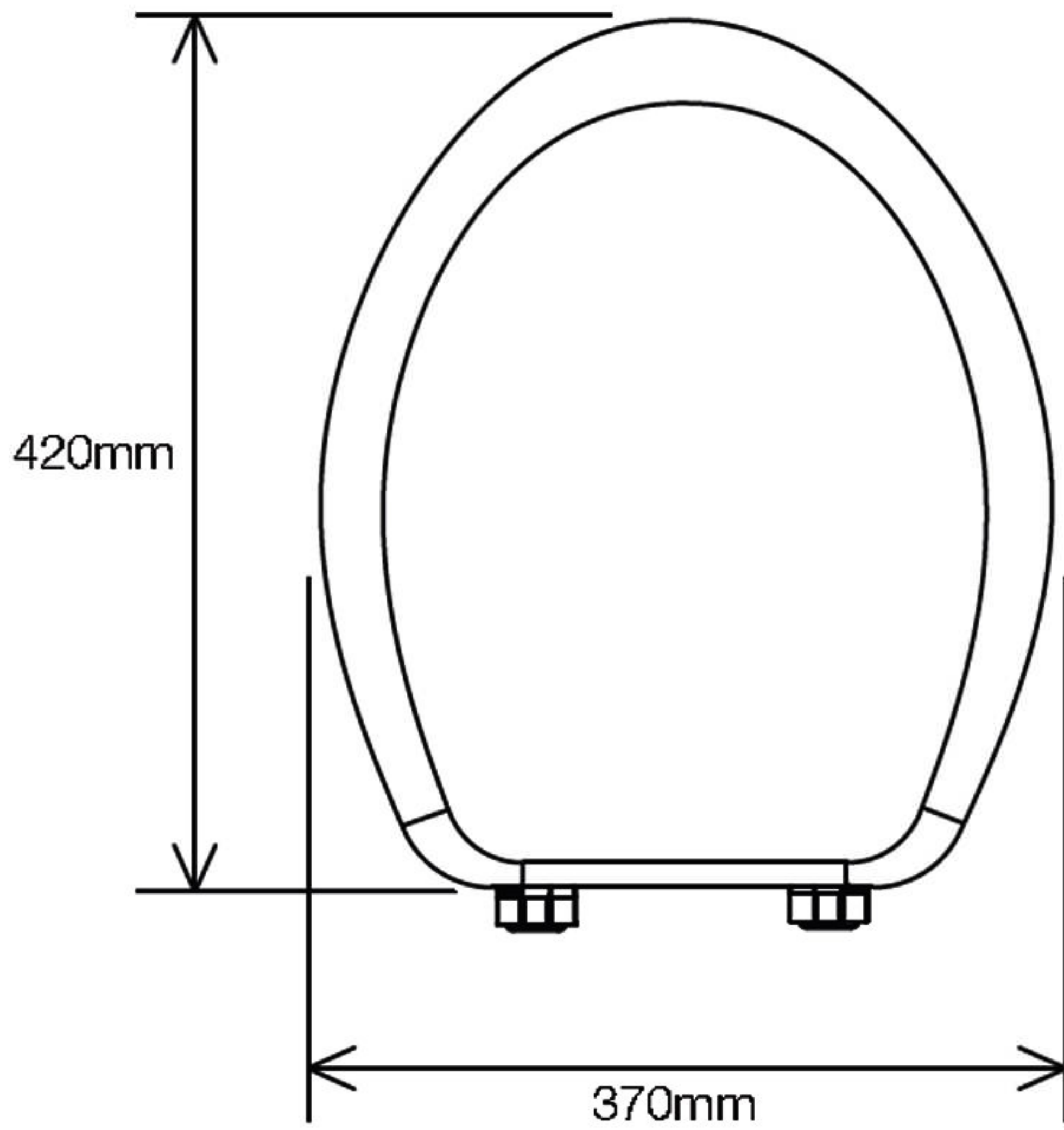
general seat dimensions
